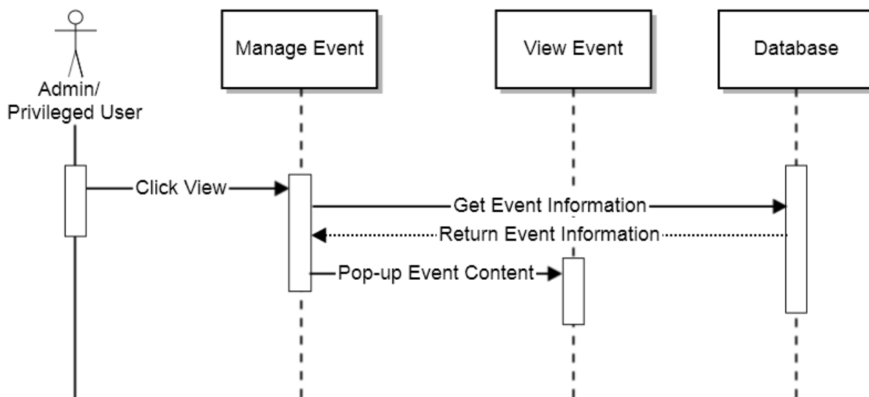
Sequence Diagram: View Event
