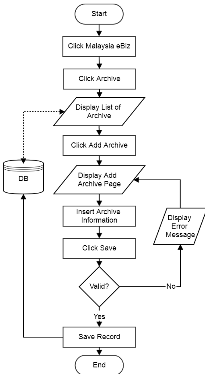
Flowchart: Add Archive
