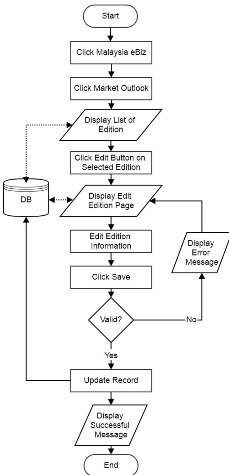
Flowchart: Edit Edition
