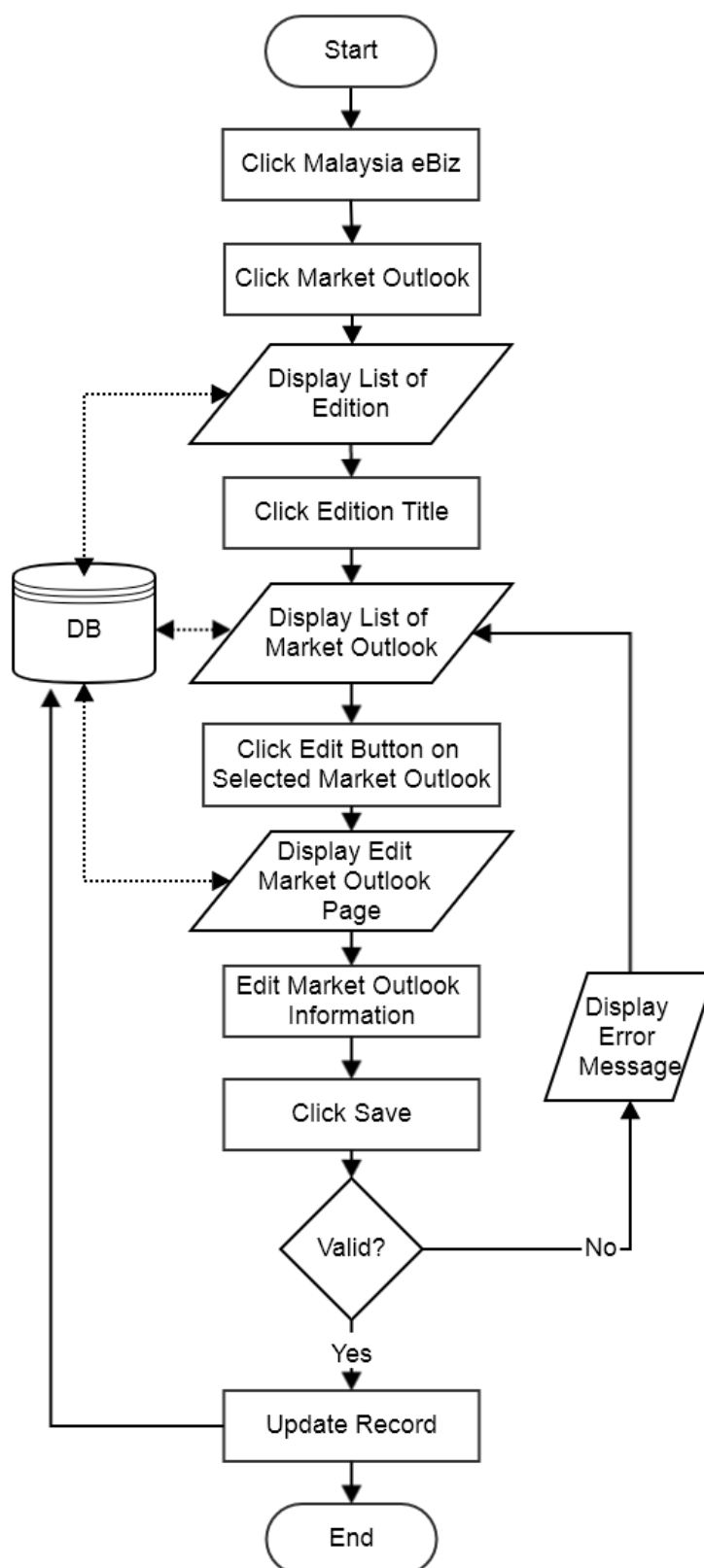
Flowchart: Edit Market Outlook
