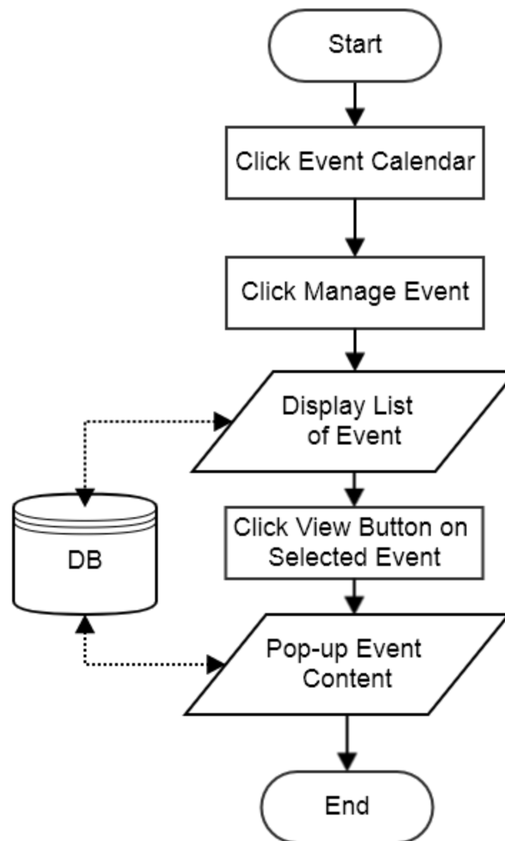
Flowchart: View Event
