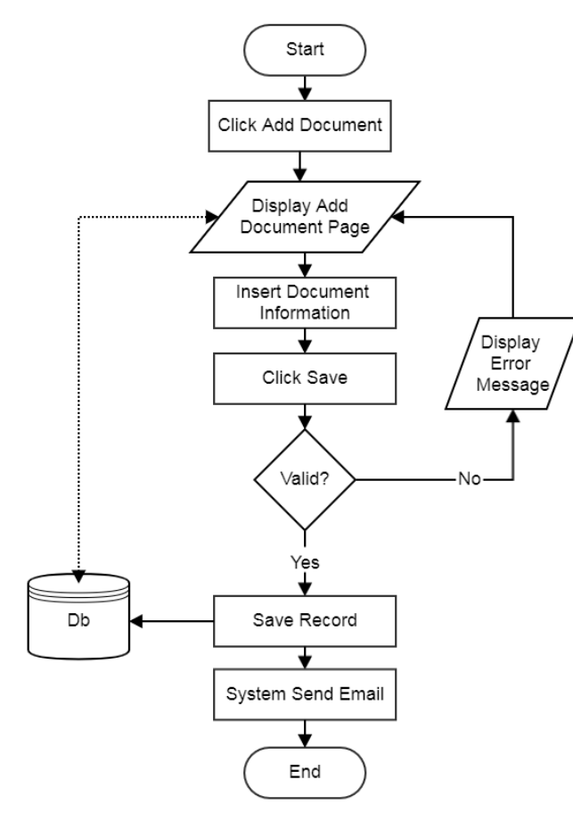
Flowchart: Add Document
