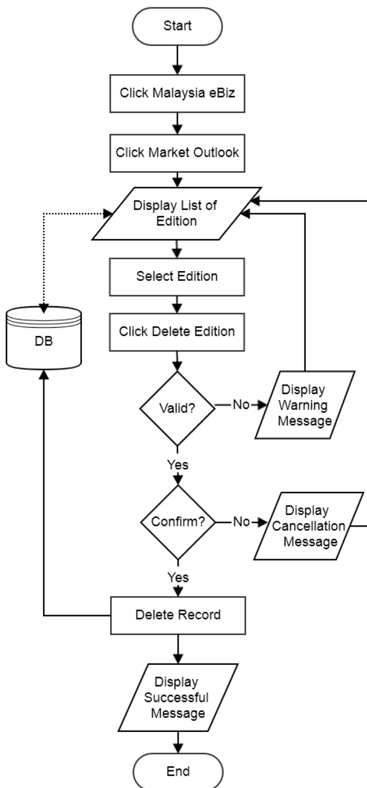
Flowchart: Delete Edition
