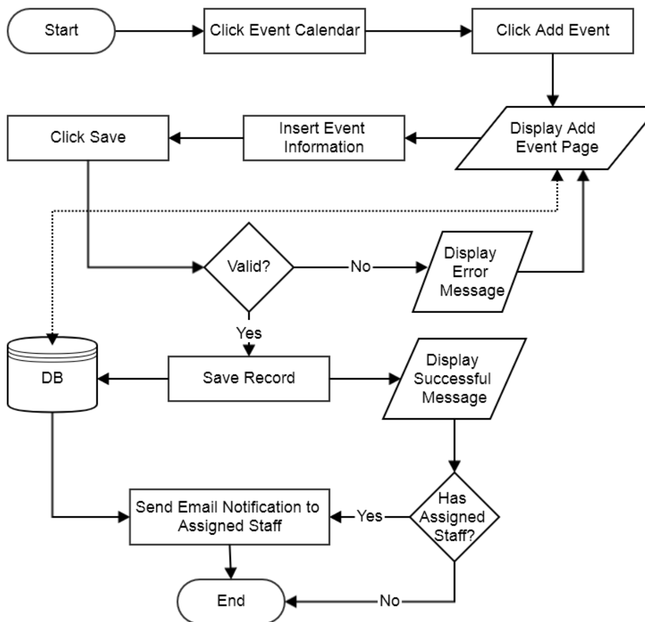
Flowchart: Add Event
