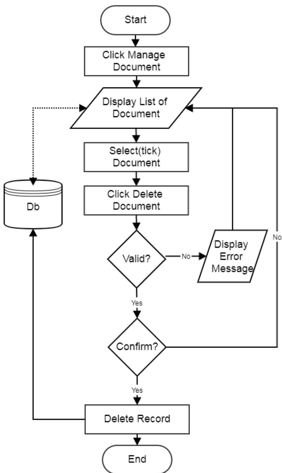
Flowchart: Delete Document
