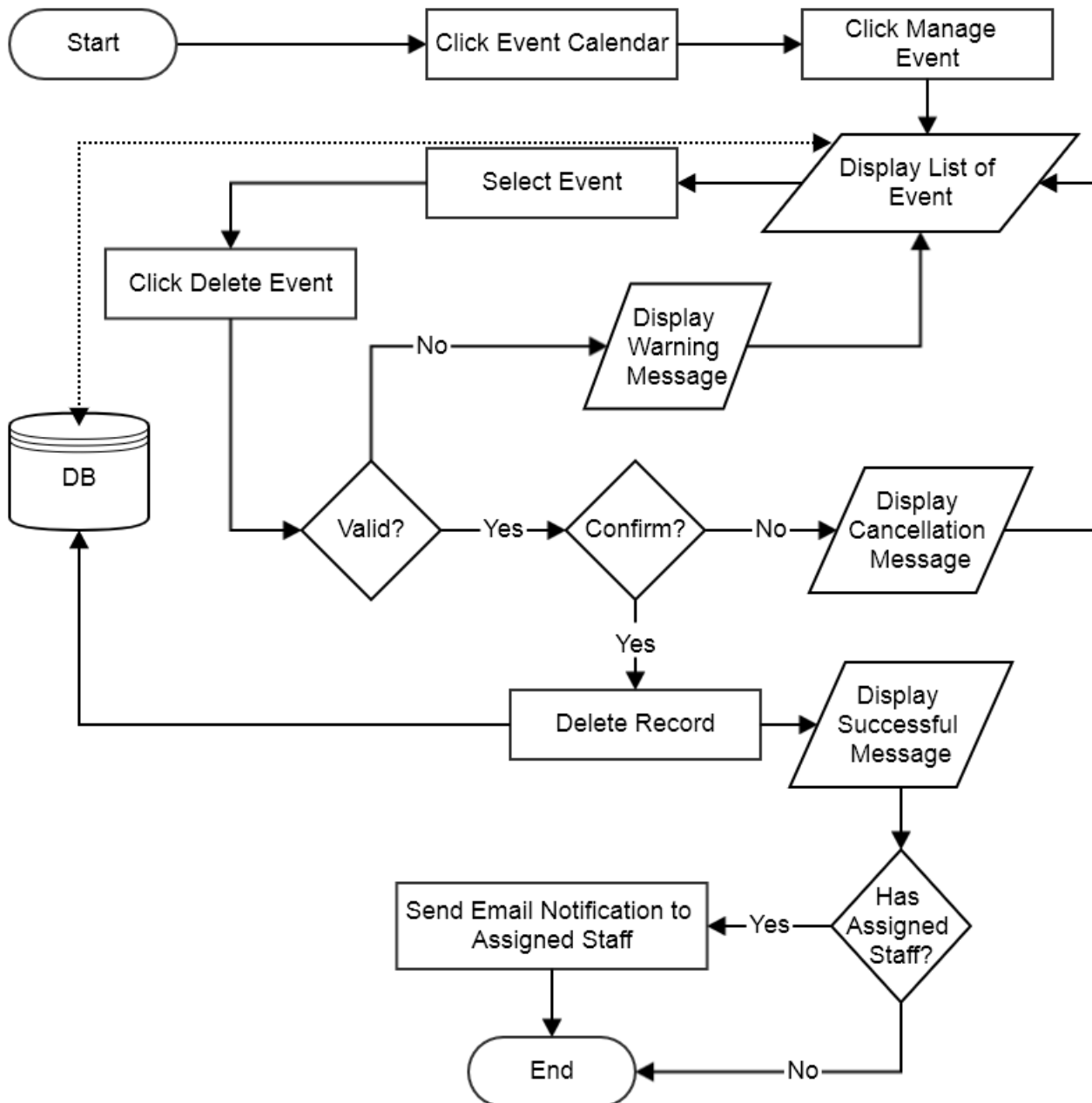
Flowchart: Delete Event
