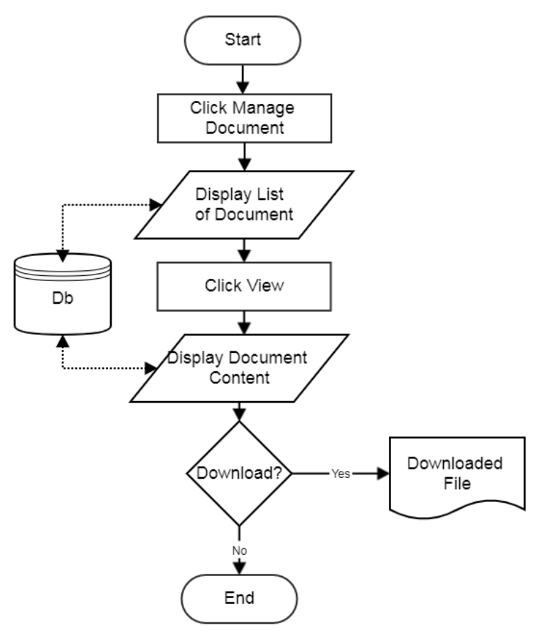
Flowchart: View Document
