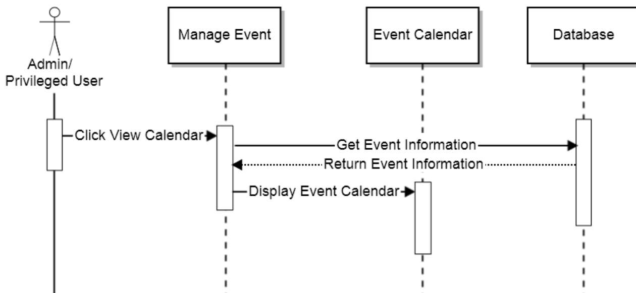
Sequence Diagram: View Calendar
