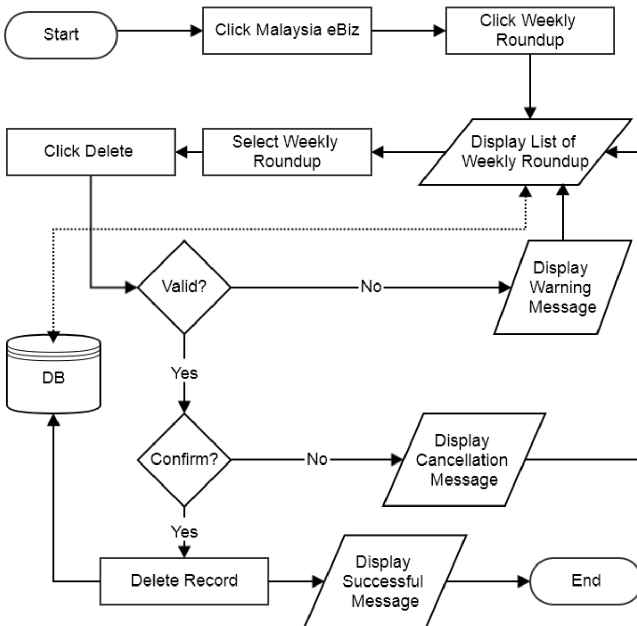
Flowchart: Delete Weekly Roundup
