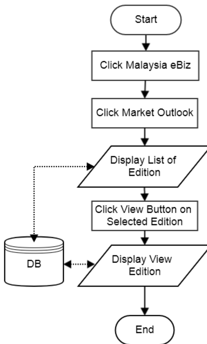
Flowchart: View Edition
