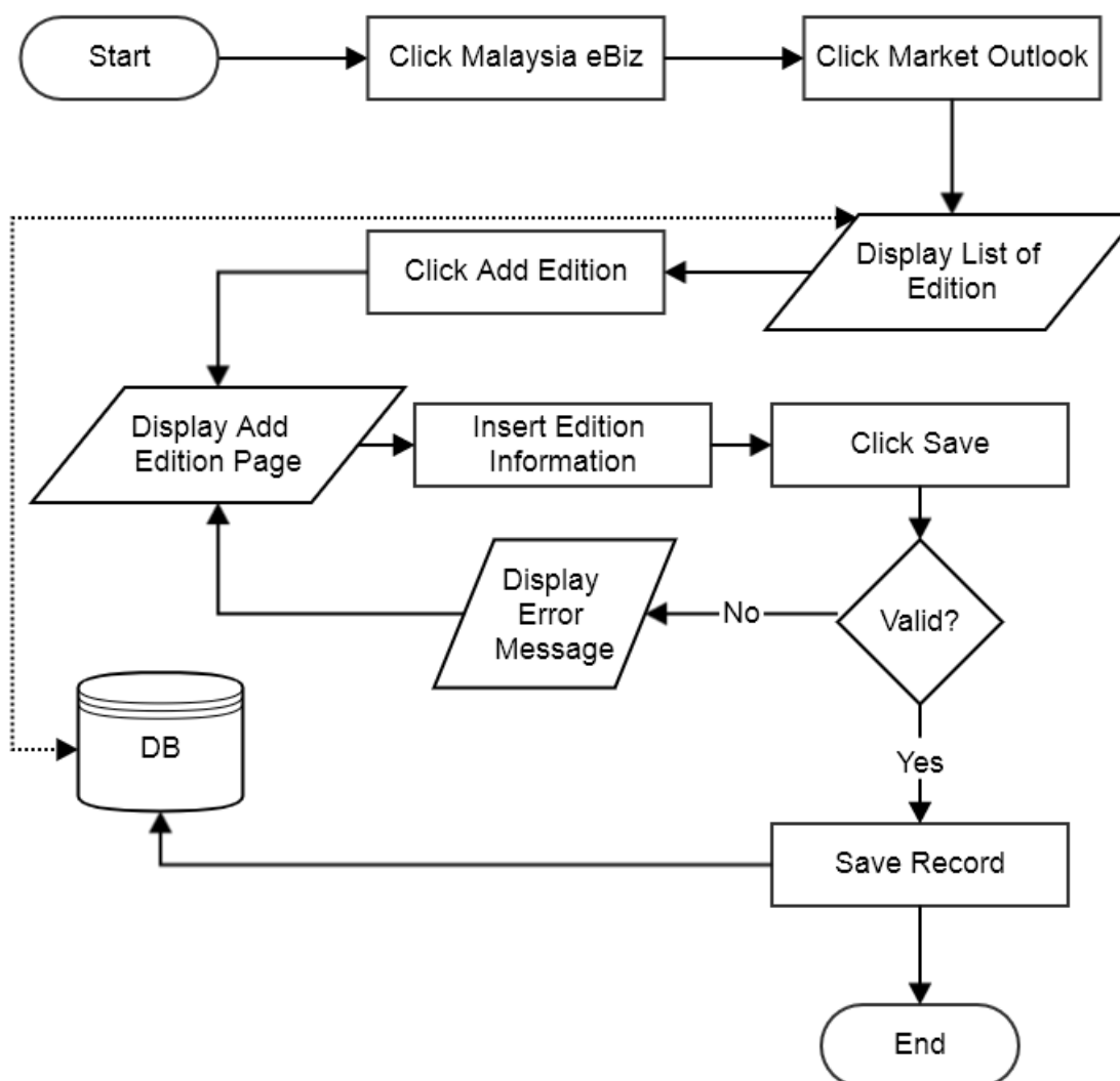
Flowchart: Add Edition
