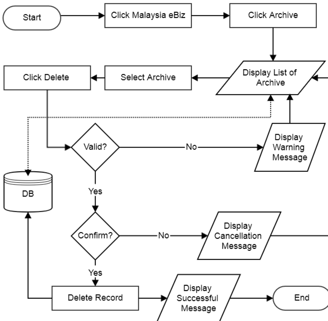
Flowchart: Delete Archive
