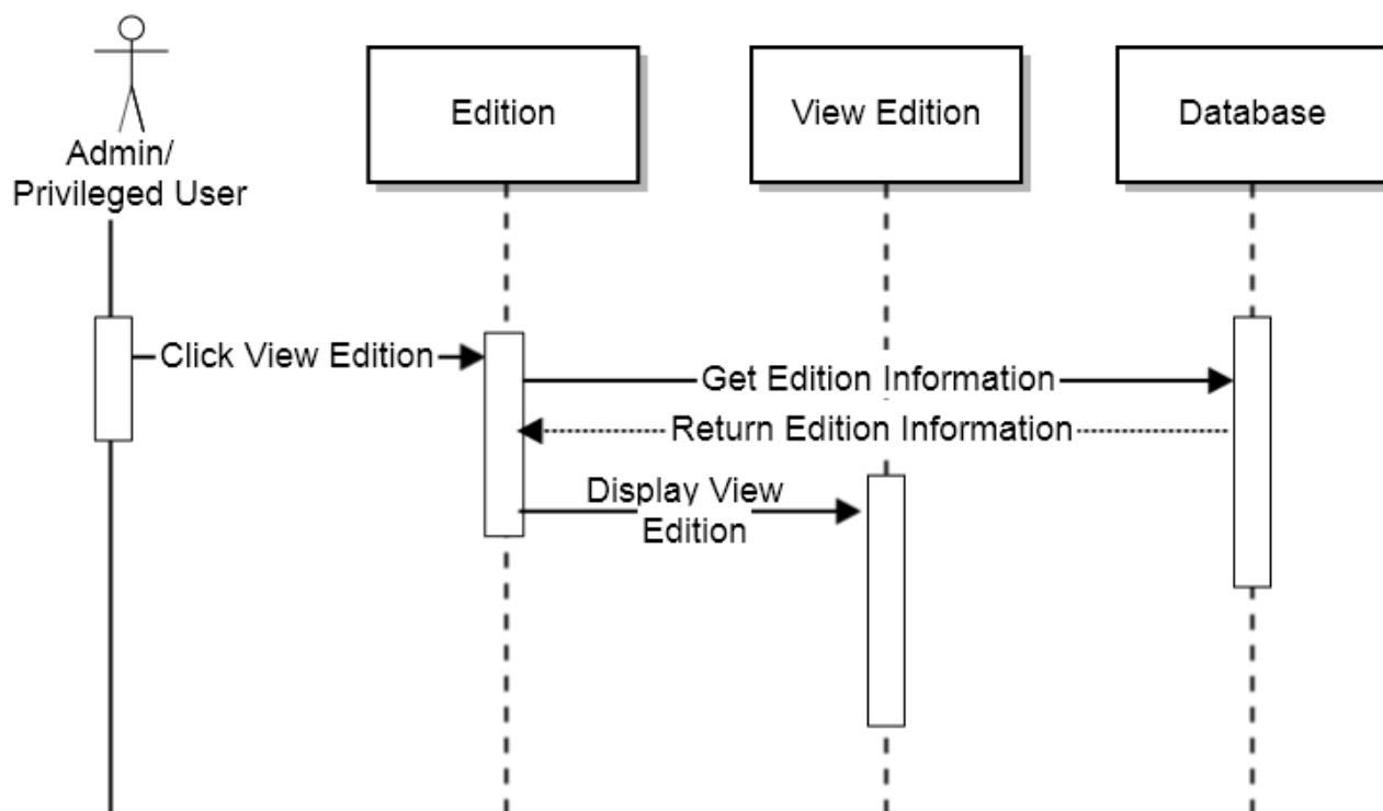
Sequence Diagram: View Edition
