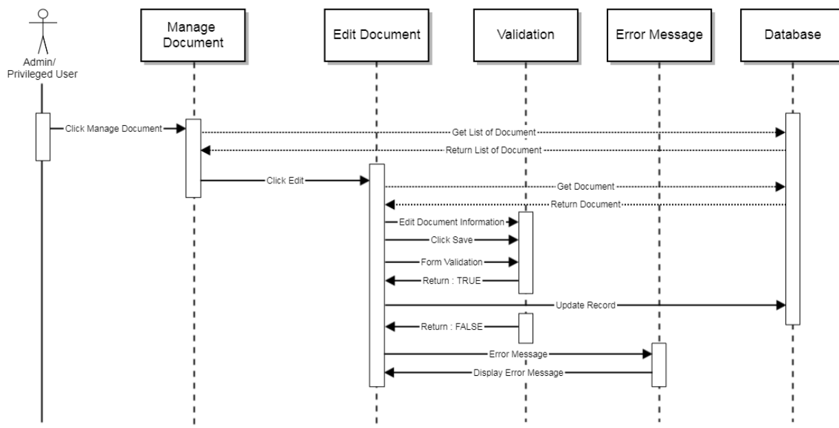
Sequence Diagram: Edit Document
