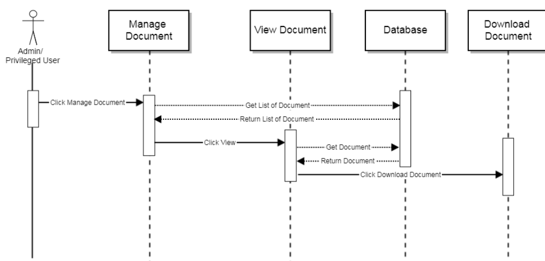
Sequence Diagram: View Document
