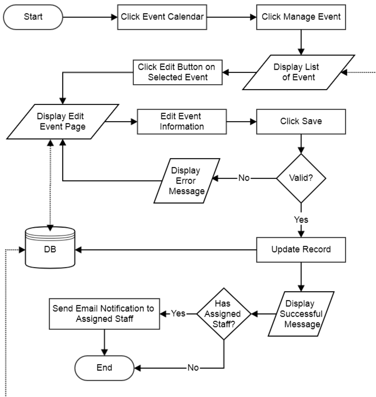
Flowchart: Edit Event
