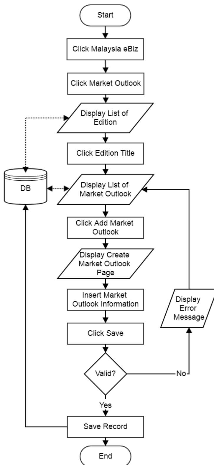
Flowchart: Add Market Outlook
