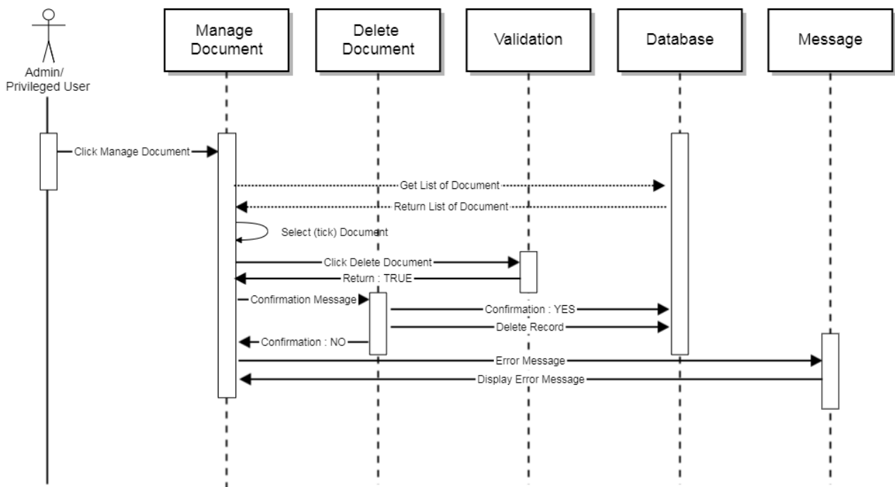
Sequence Diagram: Delete Document
