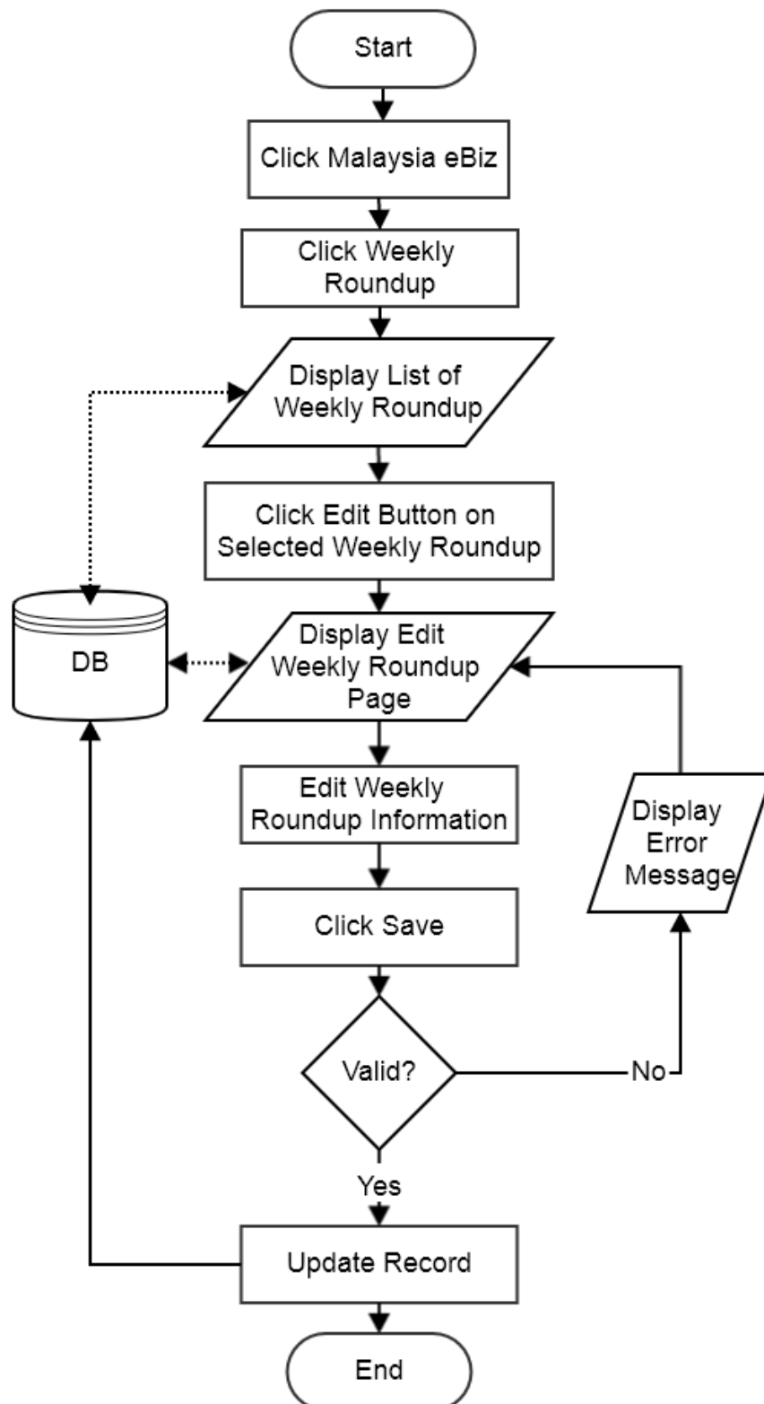
Flowchart: Edit Weekly Roundup
