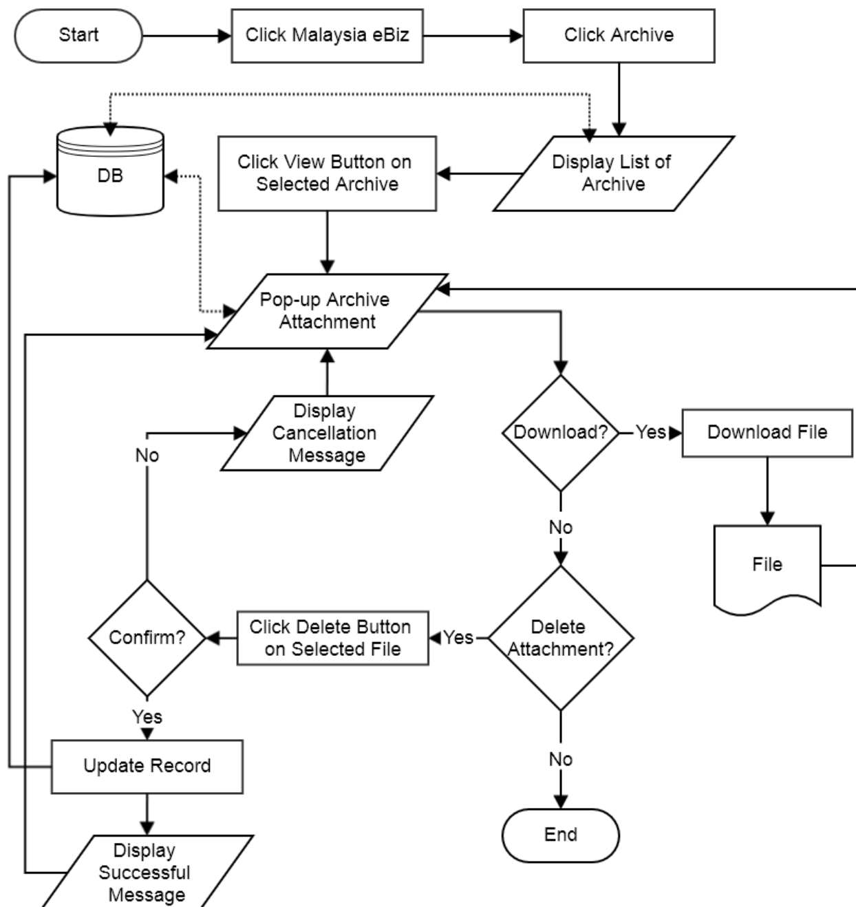
Flowchart: View Archive
