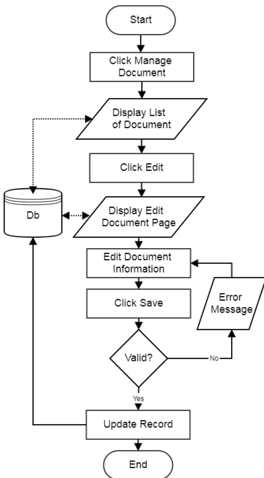
Flowchart: Edit Document
