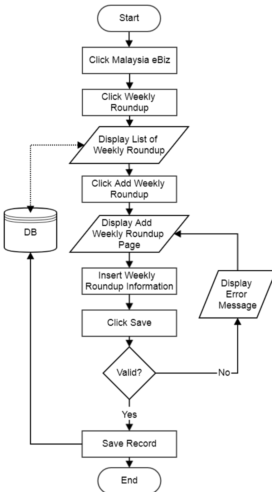
Flowchart: Add Weekly Roundup
