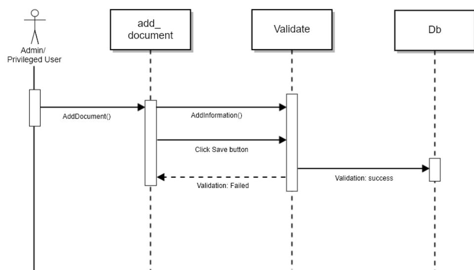
Sequence Diagram: Add Document
