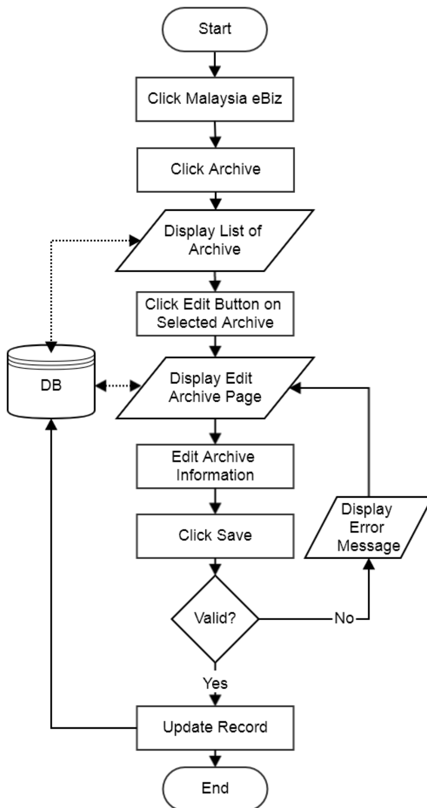
Flowchart: Edit Archive
