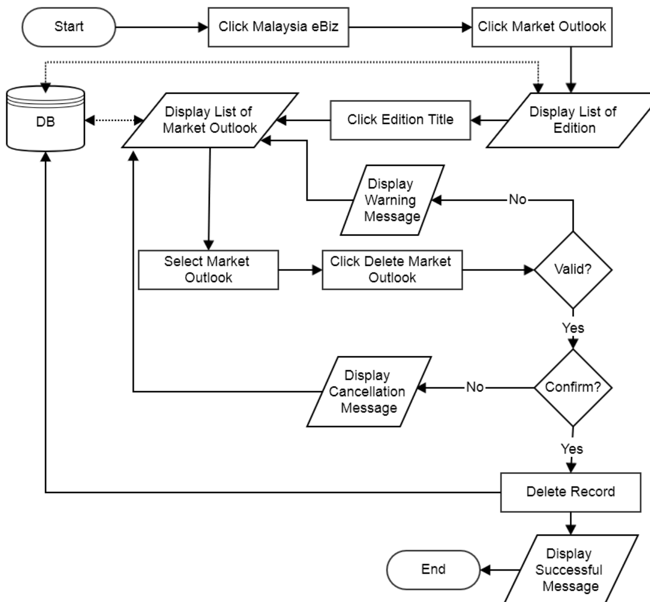
Flowchart: Delete Market
