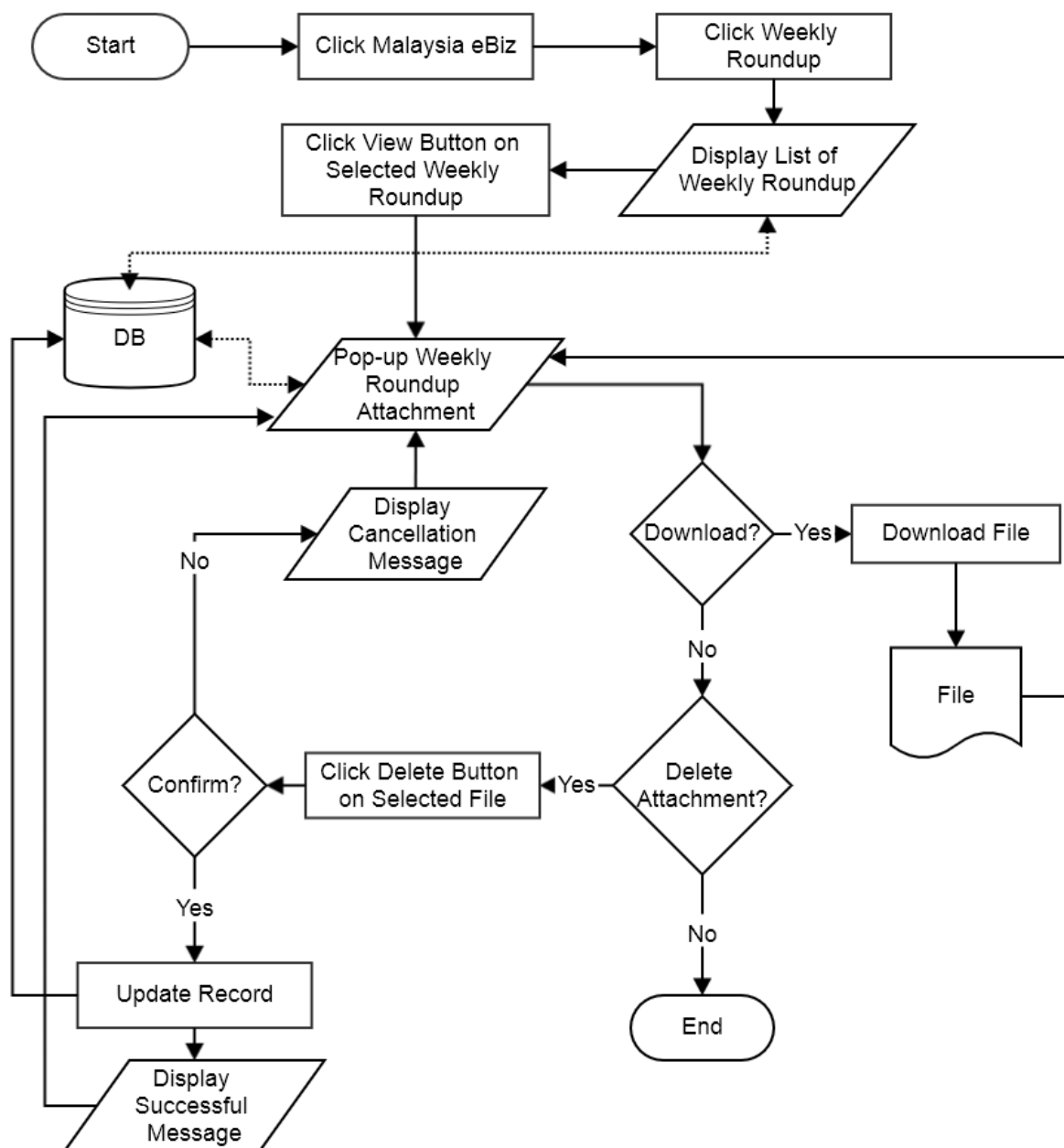
Flowchart: View Weekly Roundup
