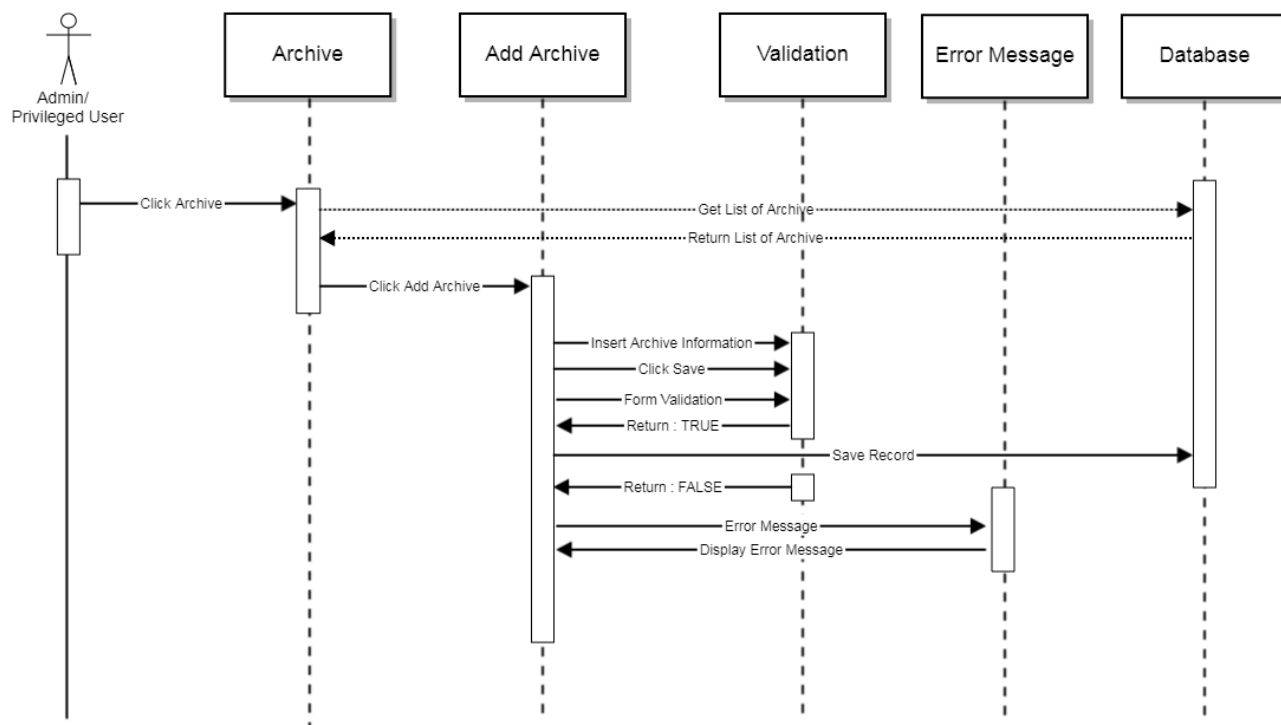
Sequence Diagram: Add Archive
