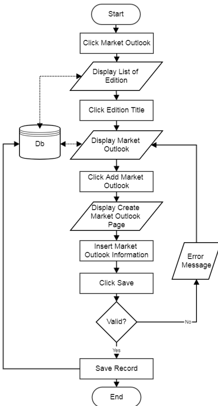
Flowchart: Add Market Outlook
