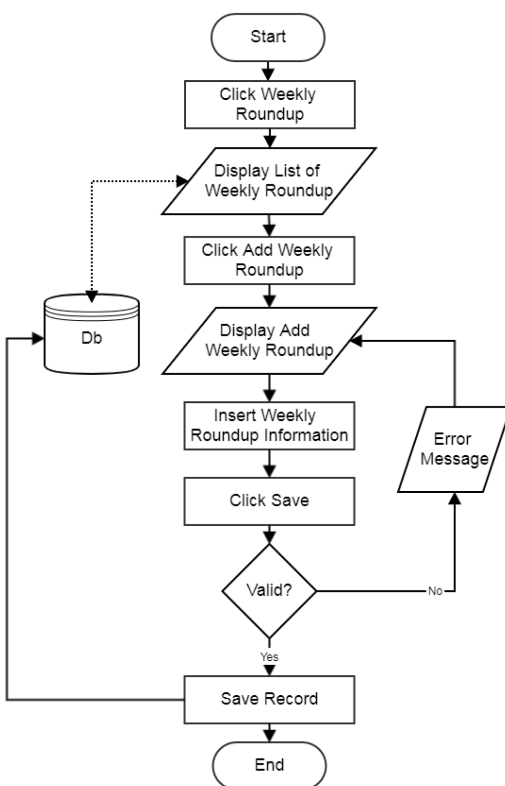
Flowchart: Add Weekly Roundup
