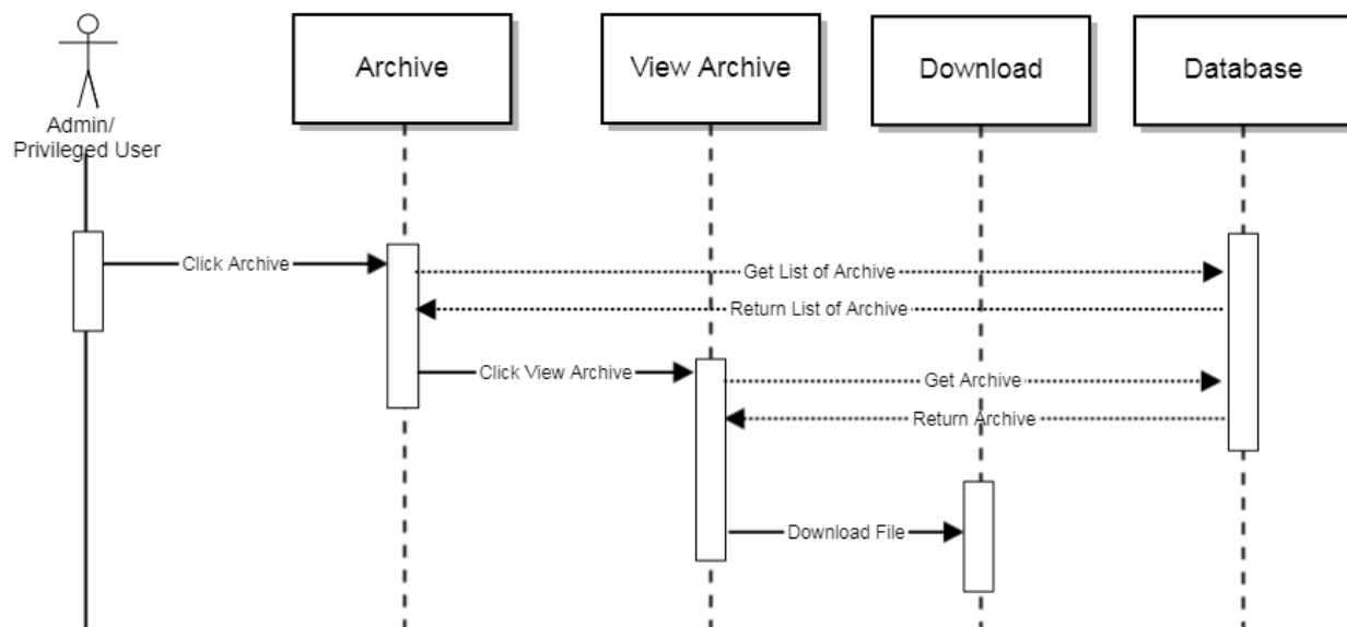
Sequence Diagram: View Archive
