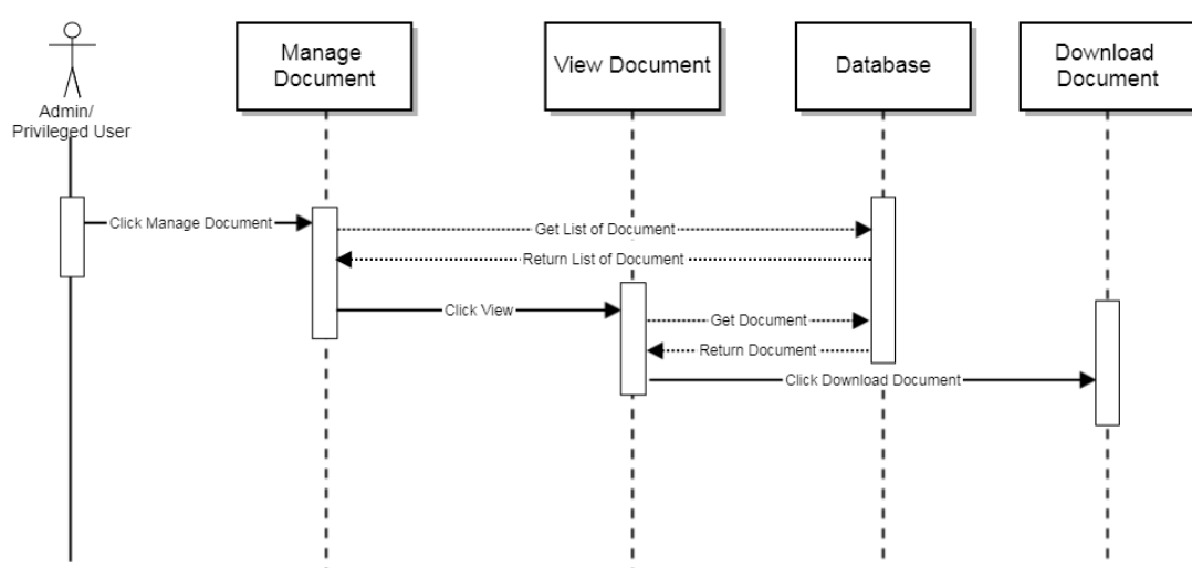
Sequence Diagram: View Document
