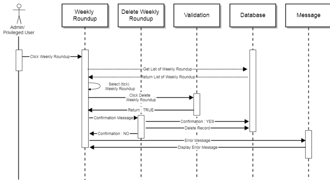
Sequence Diagram: Delete Weekly Roundup
