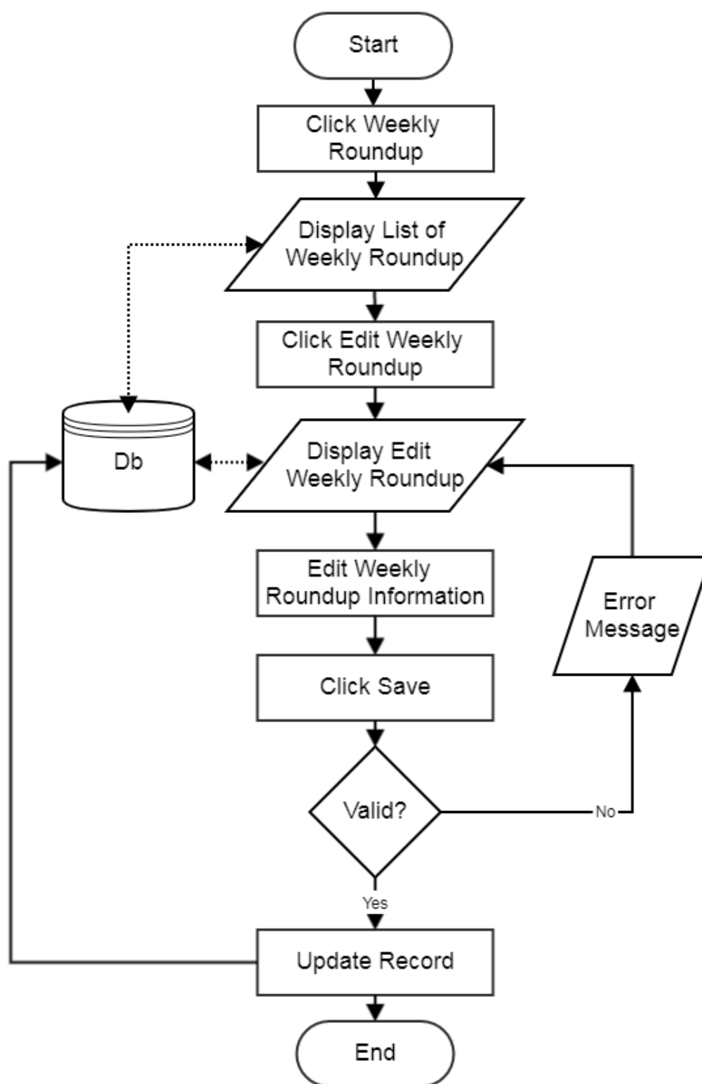
Flowchart: Edit Weekly Roundup
