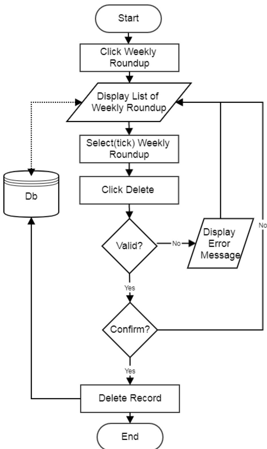
Flowchart: Delete Weekly Roundup
