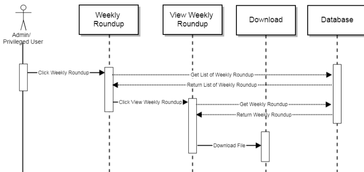
Sequence Diagram: View Weekly Roundup
