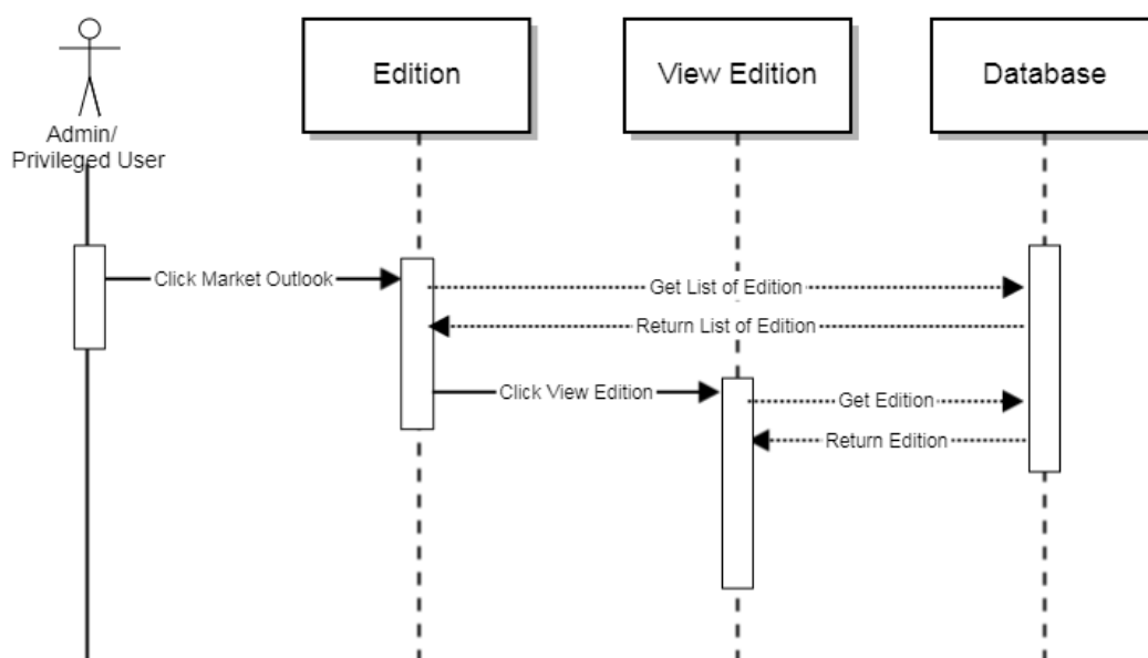
Sequence Diagram: View Edition
