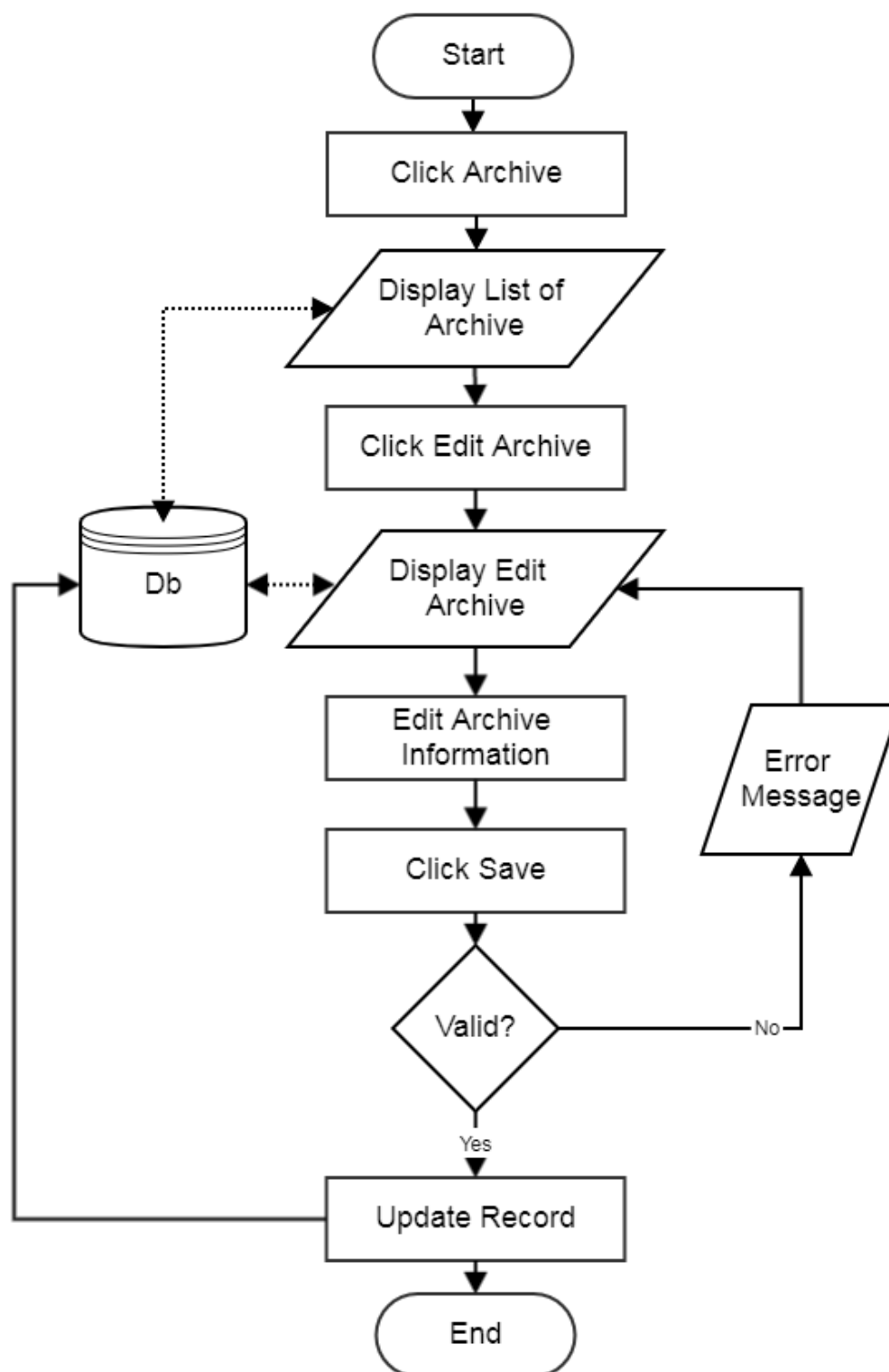
Flowchart: Edit Archive
