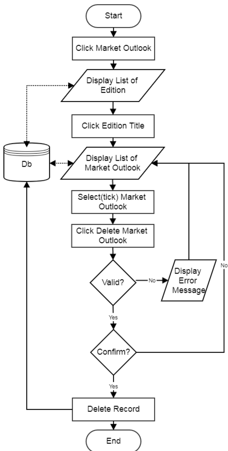
Flowchart: Delete Market
