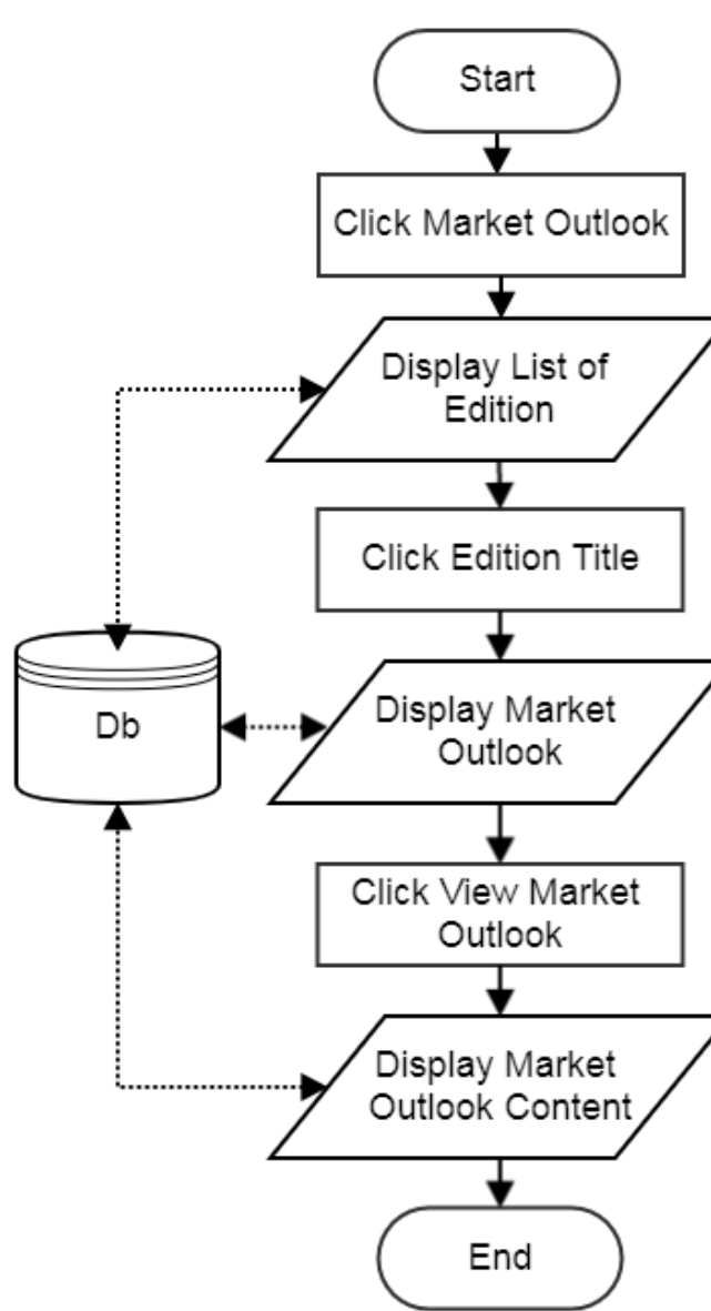
Flowchart: View Market Outlook
