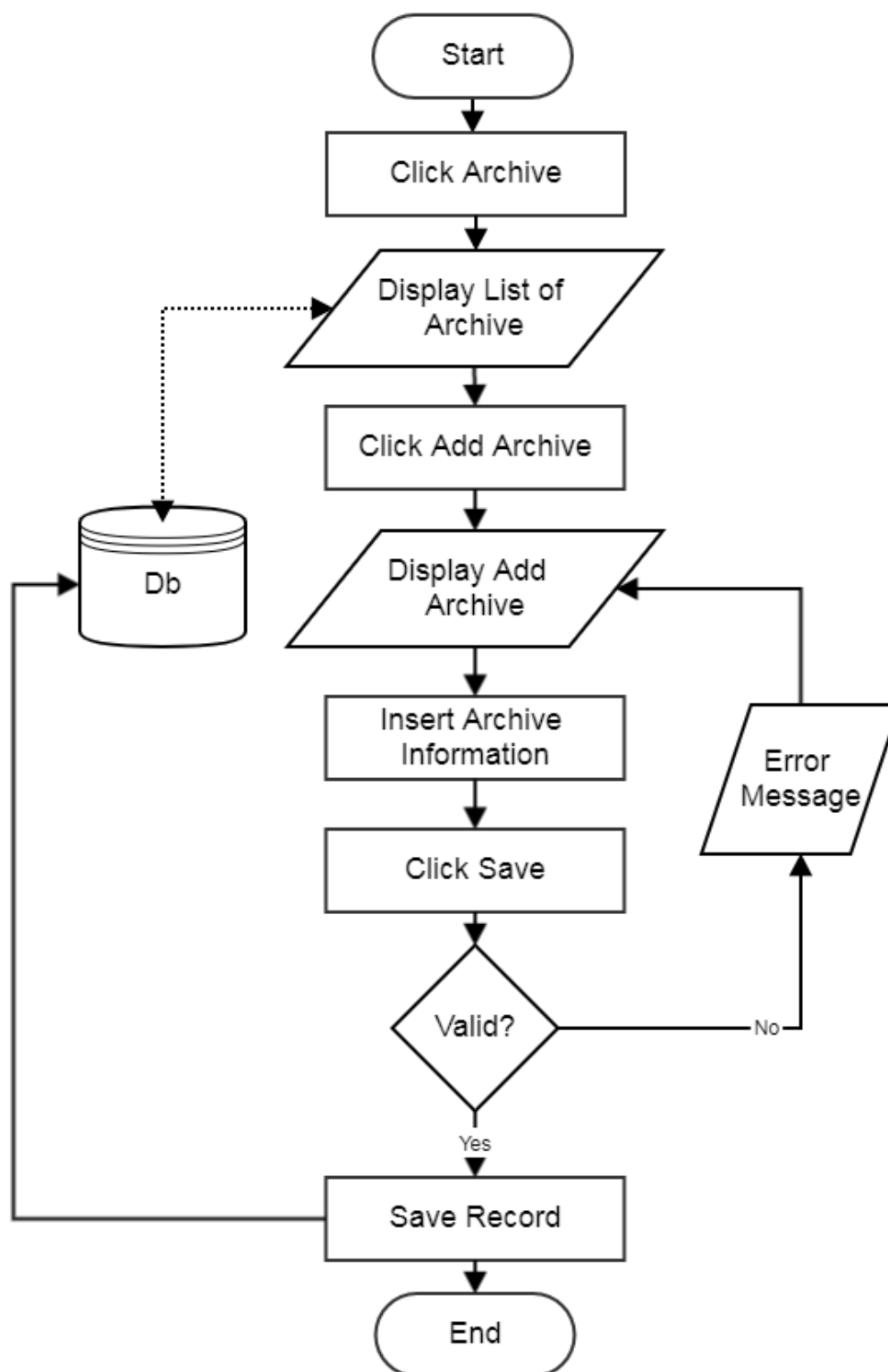
Flowchart: Add Archive
