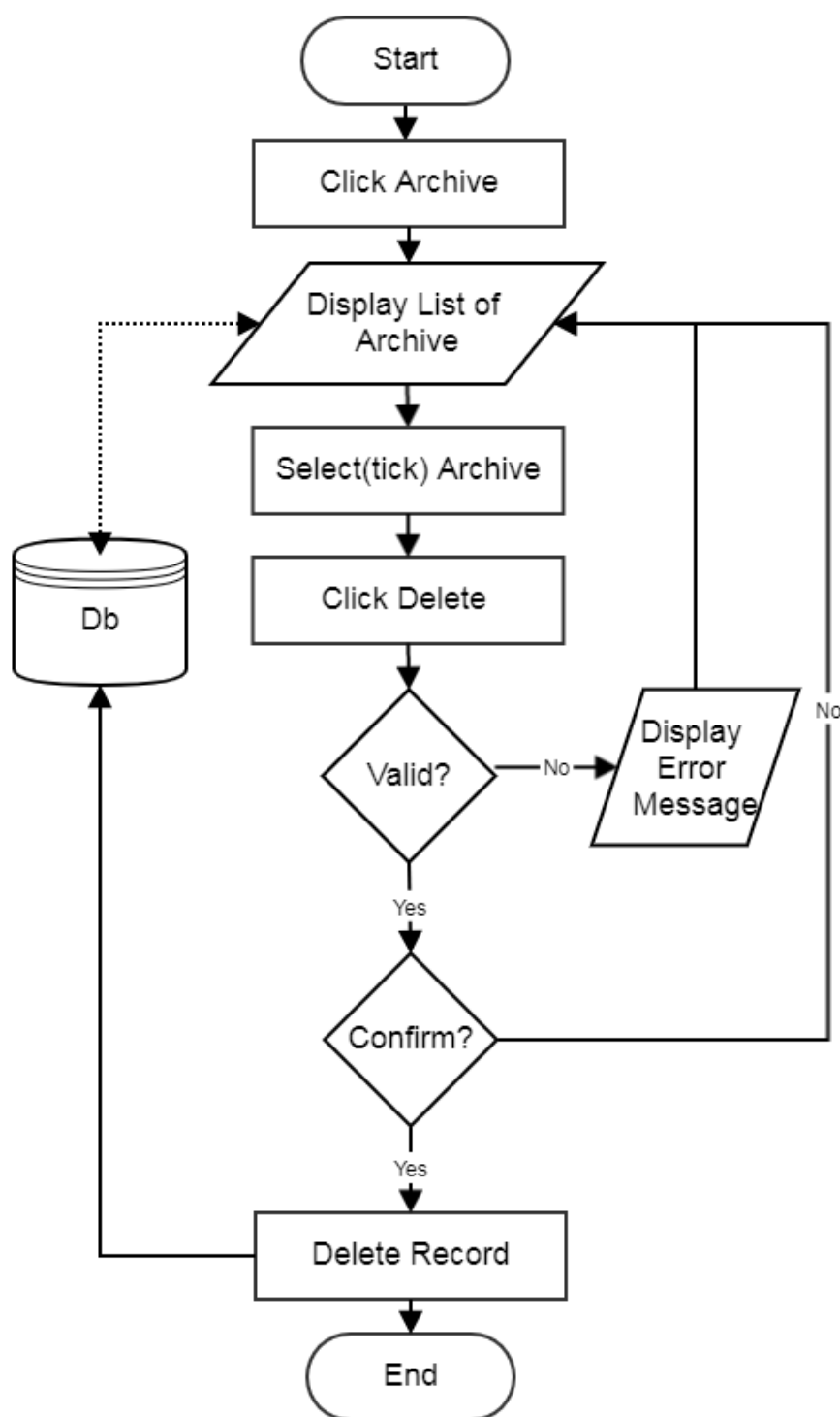
Flowchart: Delete Archive
