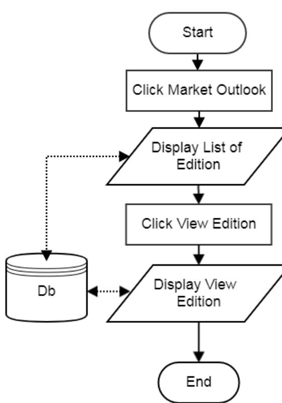
Flowchart: View Edition
