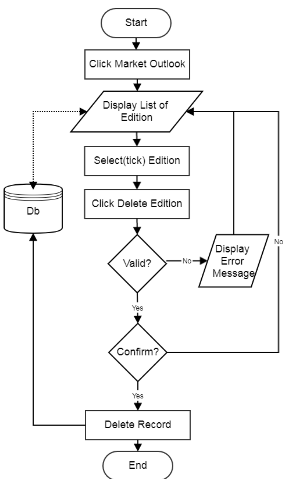
Flowchart: Delete Edition
