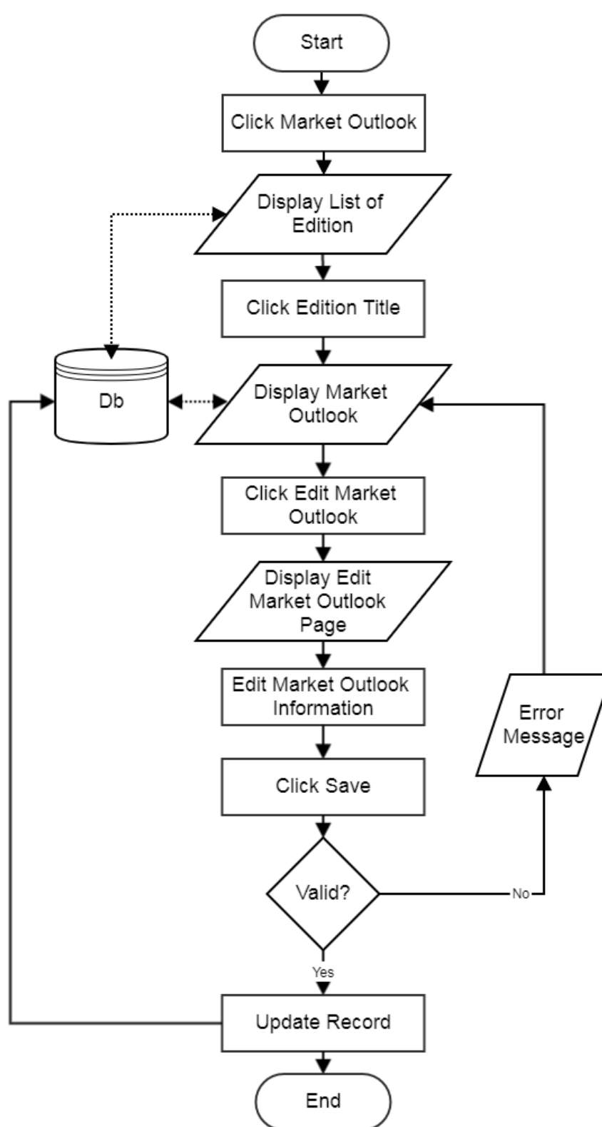
Flowchart: Edit Market Outlook
