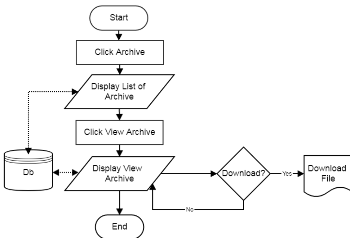
Flowchart: View Archive
